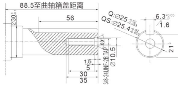
Hydraulic motor installation parameters diagram
